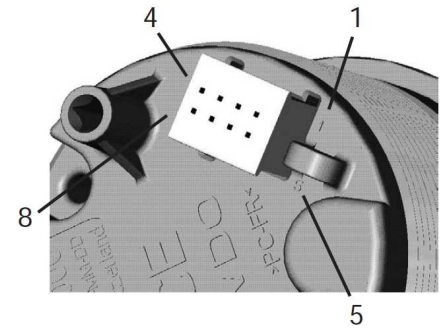
VL Flex 52 rear view Tyco / Hirschmann 8-pole MQS plug
